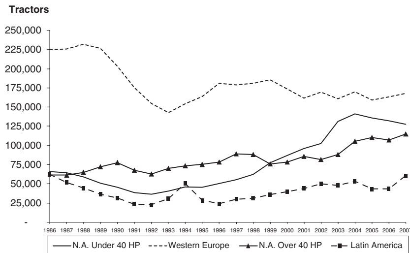
Agricultural Tractor Industry Retail Unit Sales North America, Western Europe and Latin America
